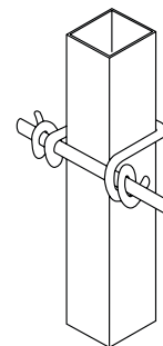
Clamp for fixing mesh to pole
